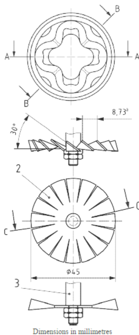
Key 1 mixer jar 2 impeller 3 mixer shaft a Horizontal distance between blades (around circumference)
